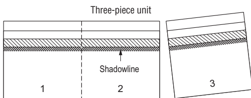
Figure 12-18: Separate to make 3 cap shingles.
